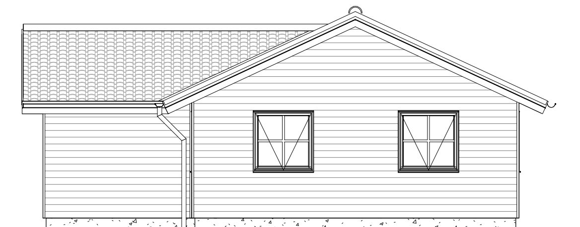
Facade 2
