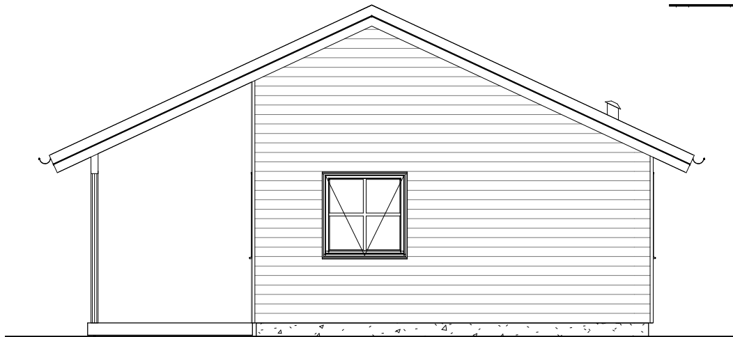
Facade 2
