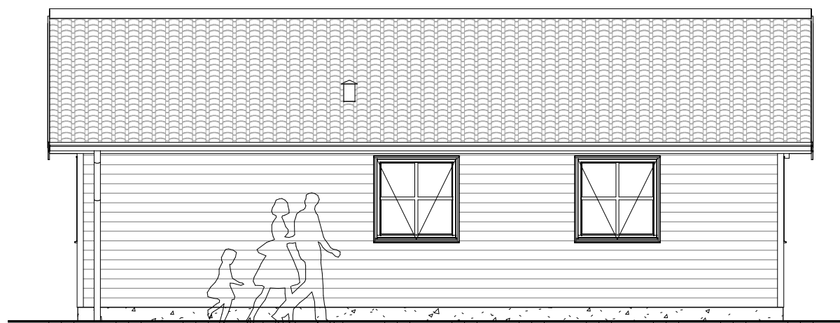
Facade 1
