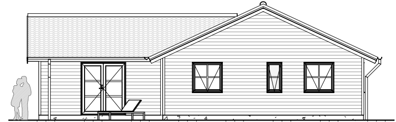
Facade 2
