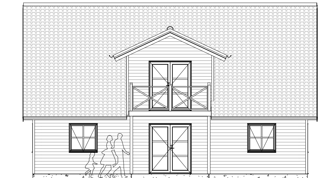
Facade 1
