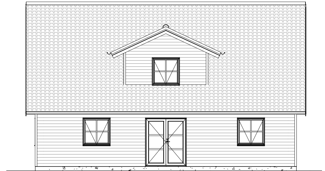
Facade 1
